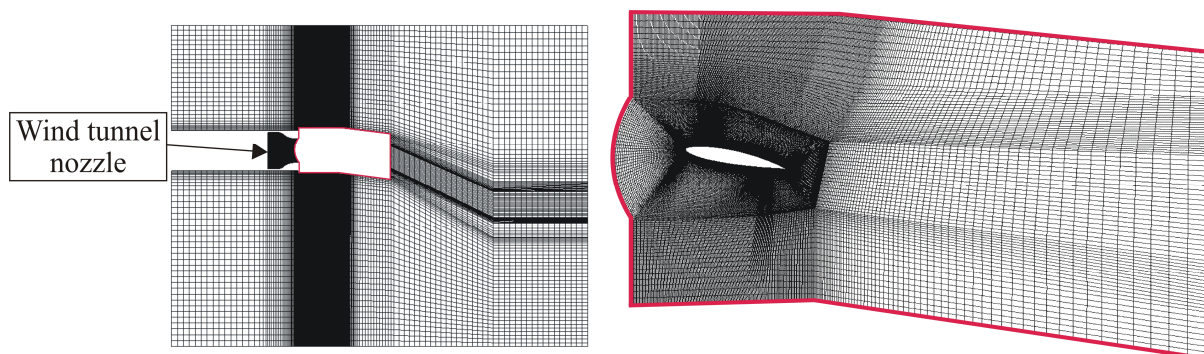
Figure 4. Computational domain and grid topology for preceding RANS of complete set up (case A, left) and for LES of the airfoil section (case B-D, right); only every 2 nd mesh line is drawn
