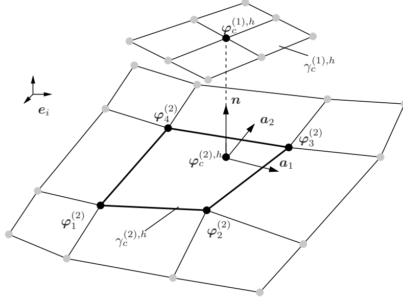
Figure 3. Three-dimensional five node NTS-element.
